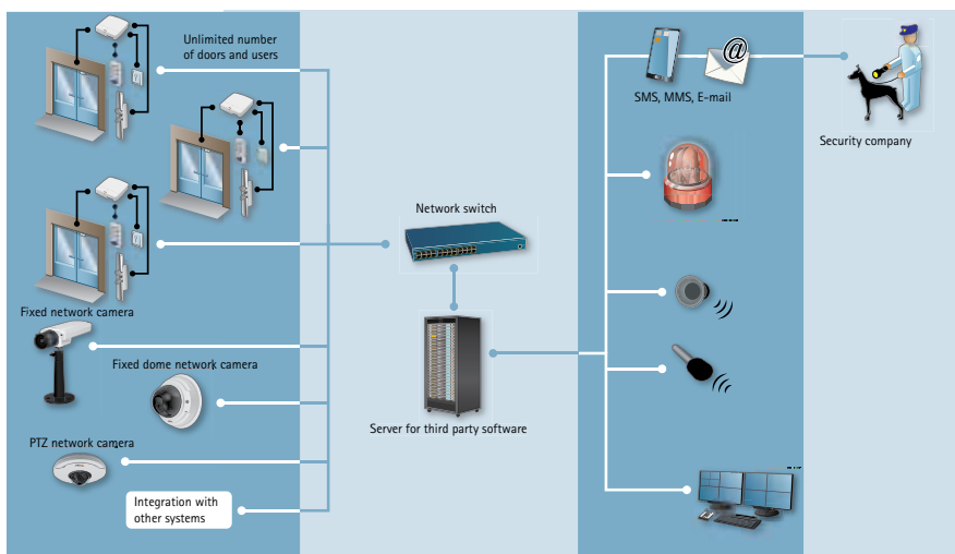
Fig 3. A schematic view of possible integrations between an access control system and a network video surveillance system and other IP-based third party applications. Note that also management functions can be distributed.
