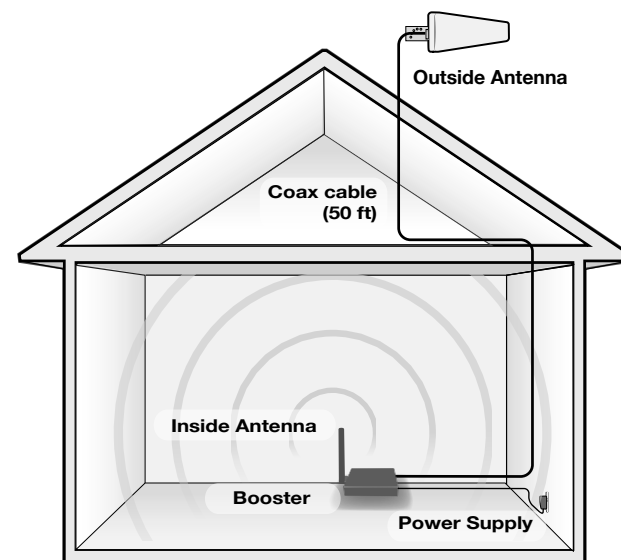
Install Overview
