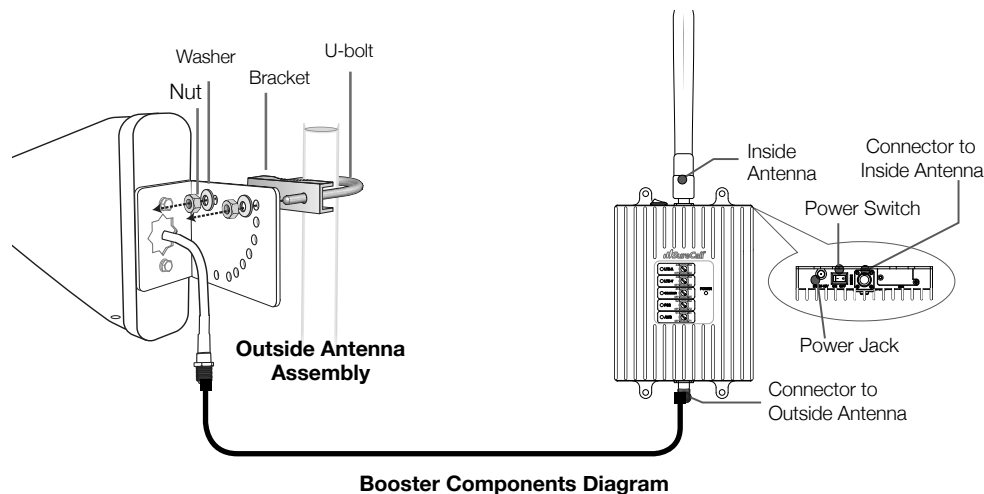
Booster Components Diagram
