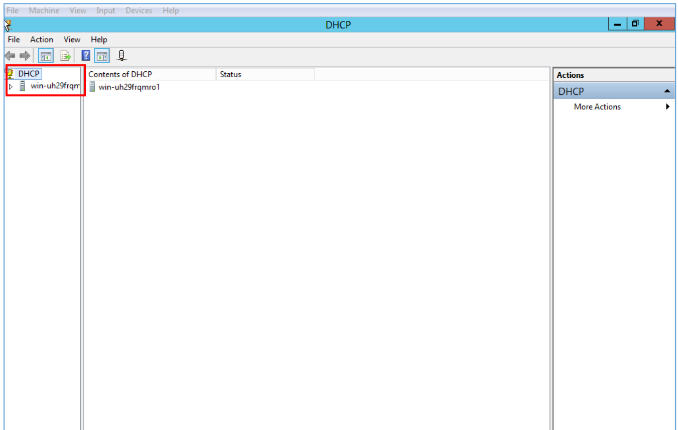
Figure 2: DHCP Management
