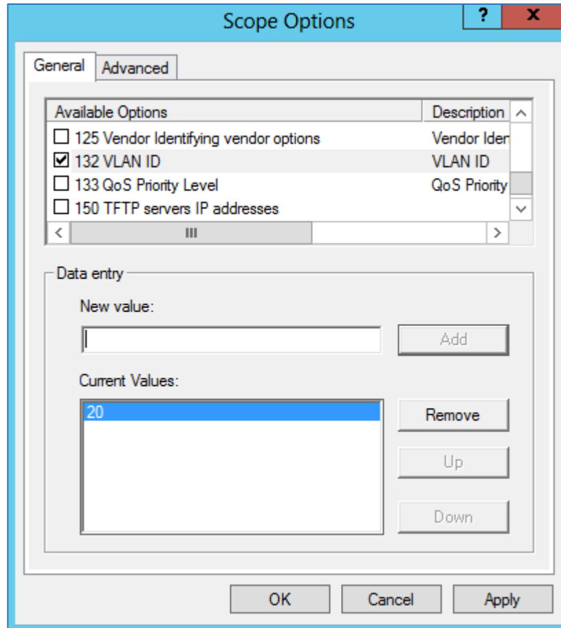
Figure 31: DHCP Option 132
