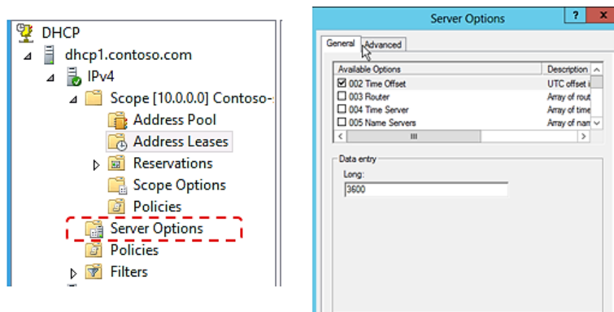
Figure 7 : Server Options
