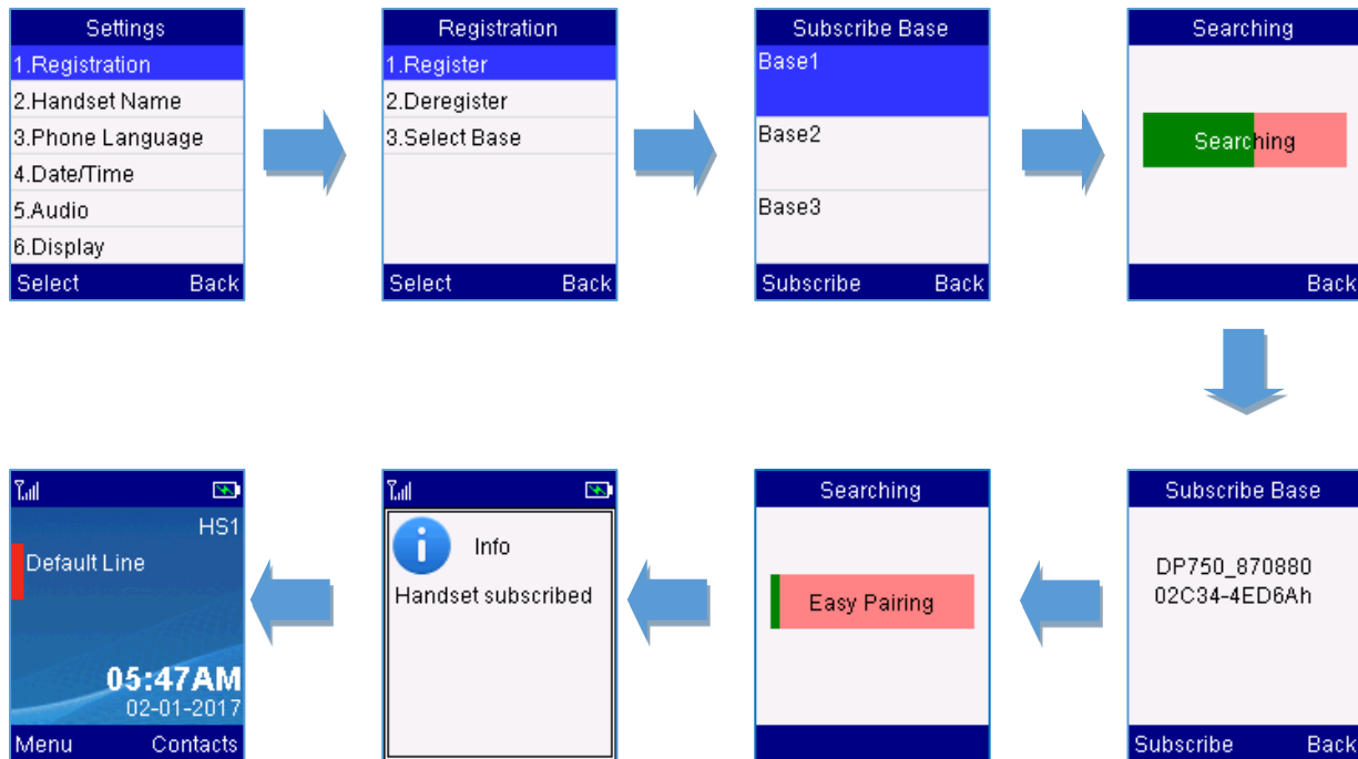
Figure 16: Registration Process
