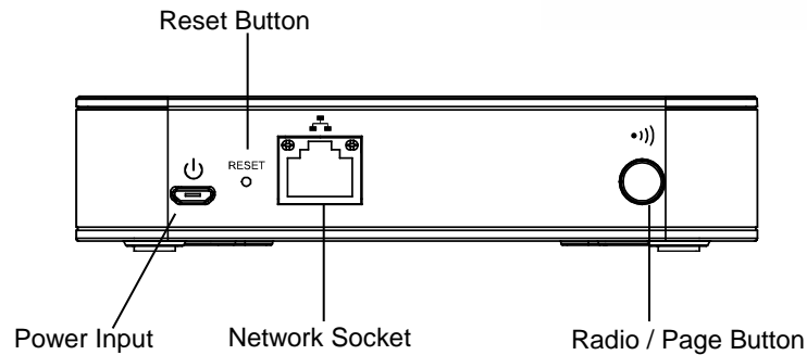
Figure 3: DP750 Back View
