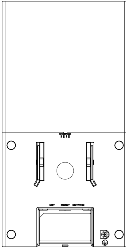
Figure 2: GWN7600LR Ports
