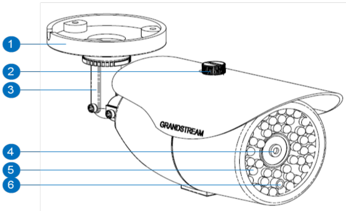
Figure 1: GXV3672_HD/FHD v2 Illustration
