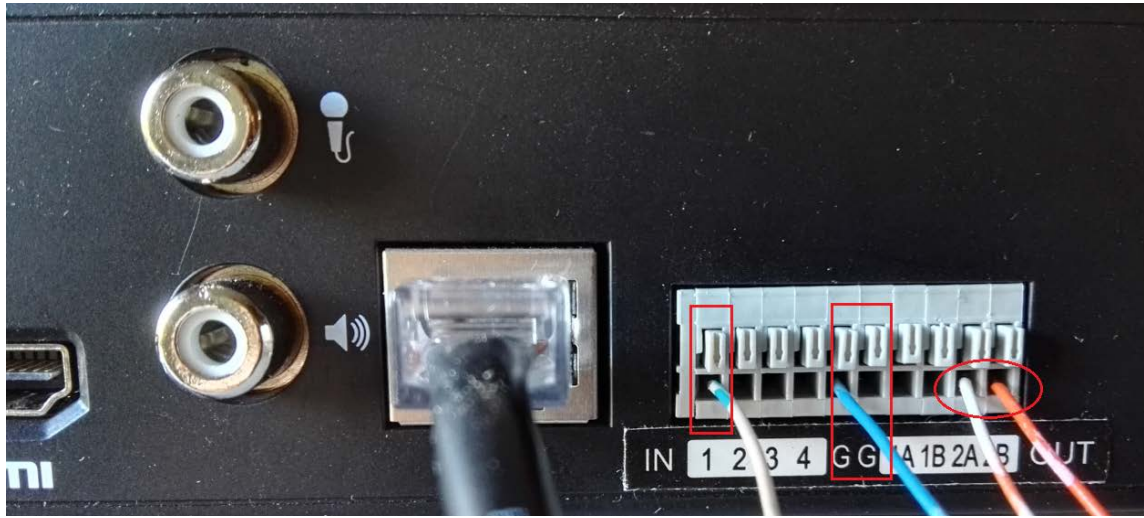
Figure 25-3: Alarm_In and Alarm_Out Wiring Diagram for GVR355X
