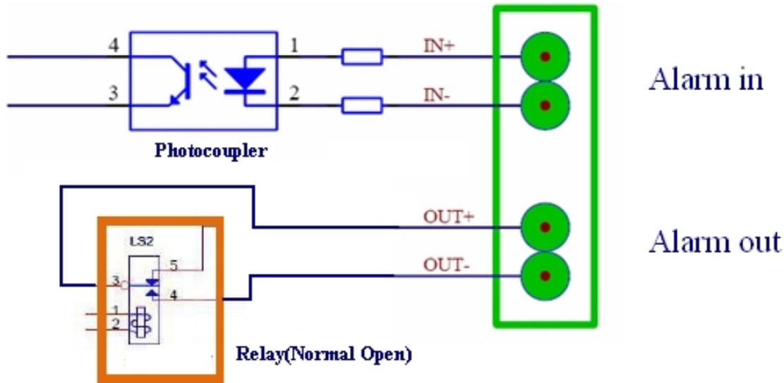
Figure 25-2: Alarm_In and Alarm_Out Connection Circuit Sample for GVR355X
