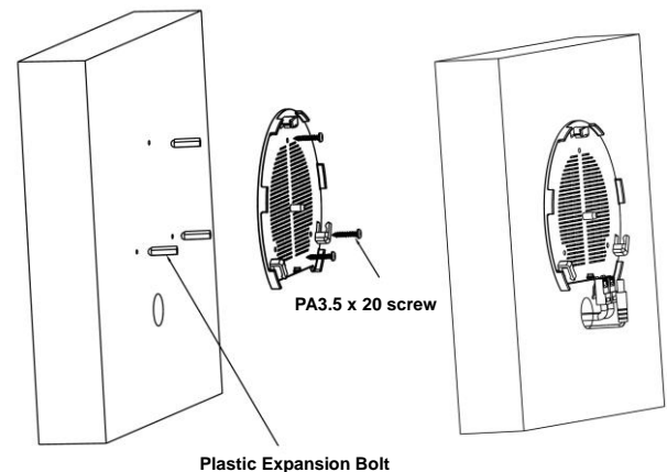
Plastic Expansion Bolt
