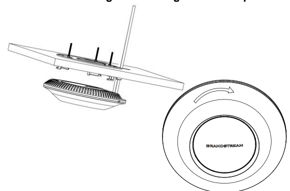
Figure 9: Ceiling Mount – Steps 5 & 6
