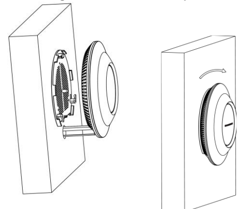
Figure 5: Wall Mount – Steps 5 & 6
