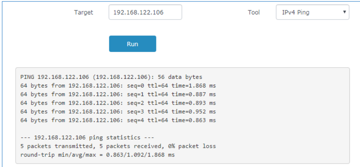
Figure 50: IP Ping
