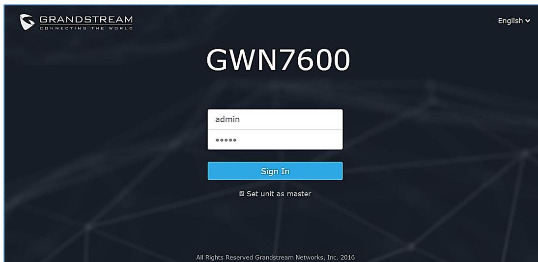
Figure 18: Login Page
