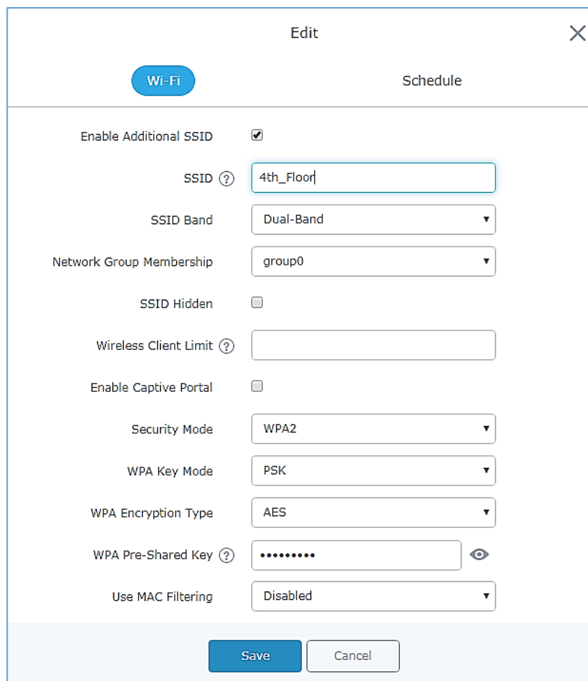
Figure 31: Additional SSID
