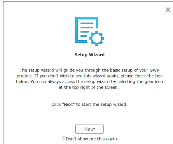
Figure 19: Setup Wizard
