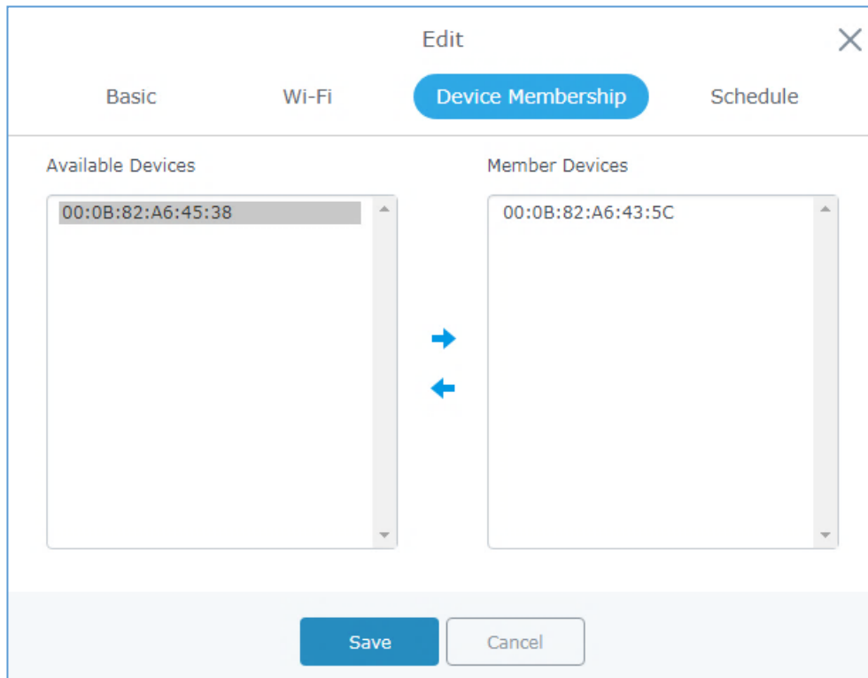
Figure 28: Device Membership
