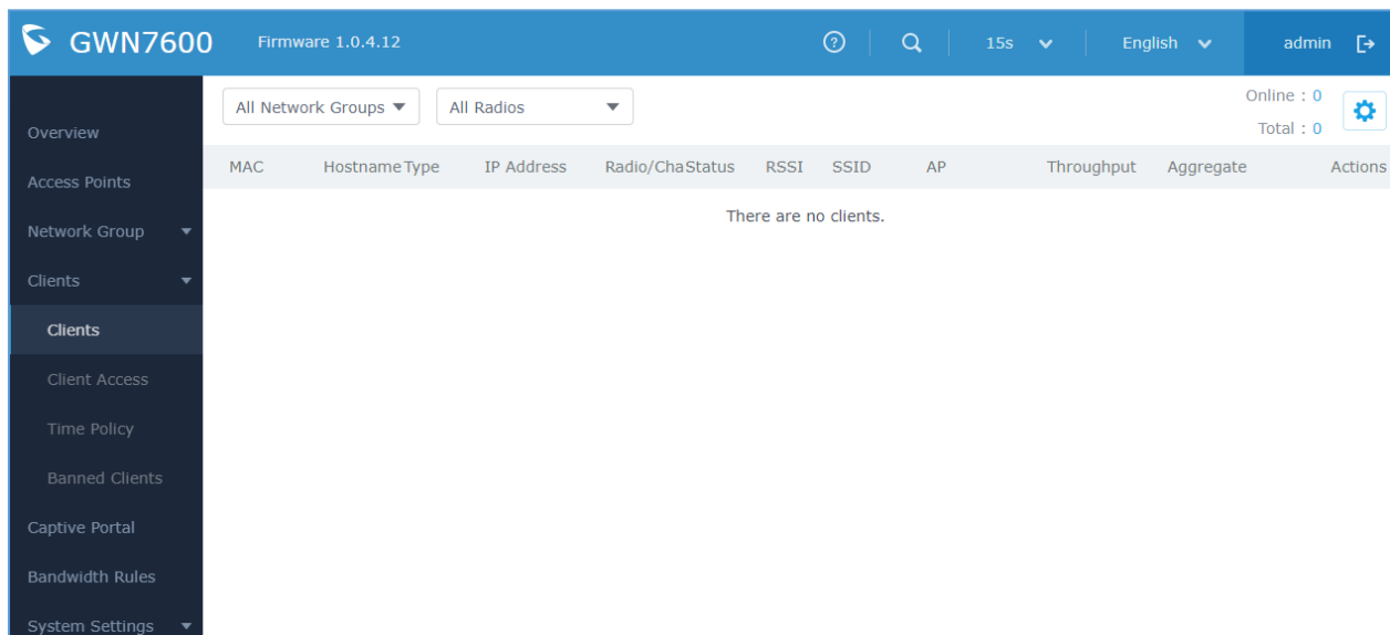
Figure 33: Clients
