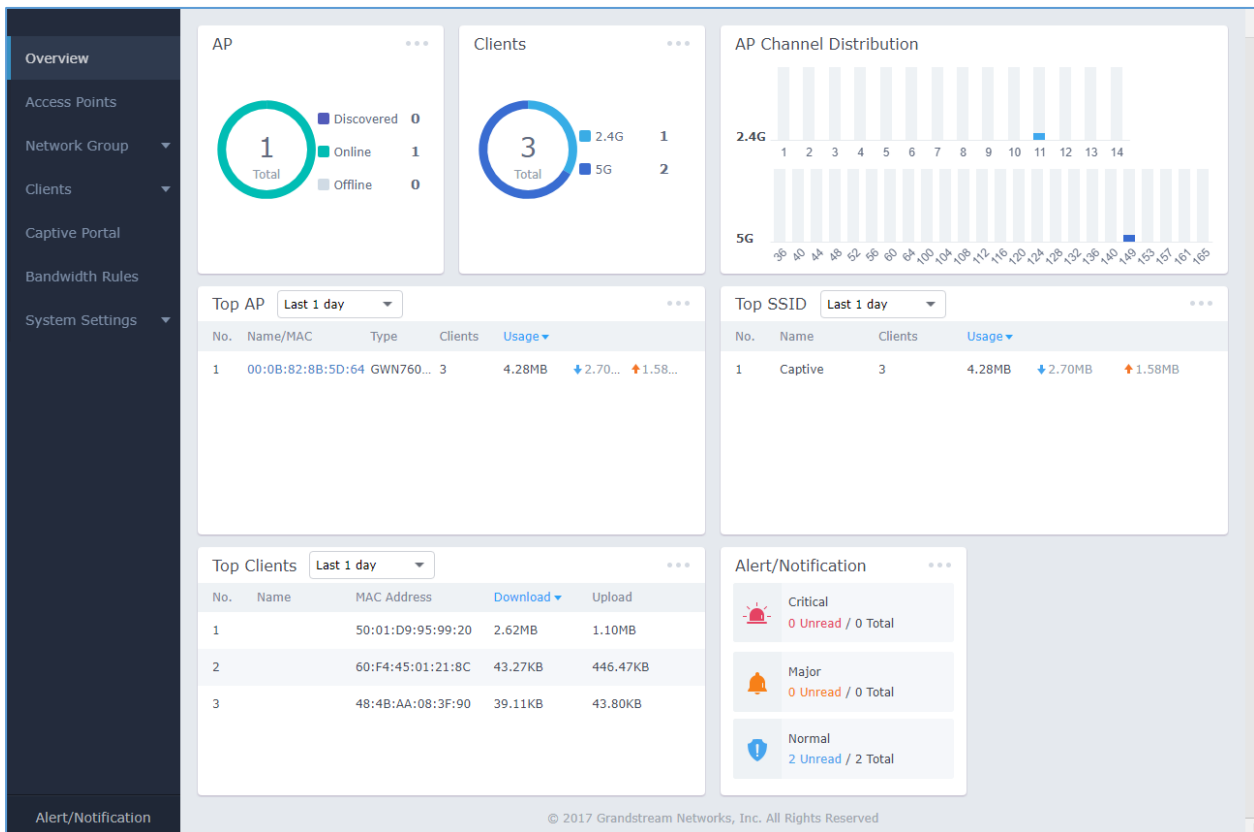
Figure 15: GWN7600's Dashboard
