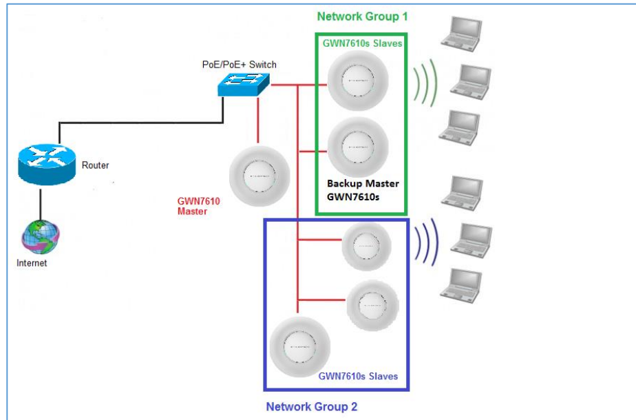
Figure 23: Failover Master
