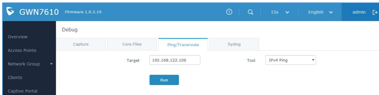
Figure 51: IP Traceroute
