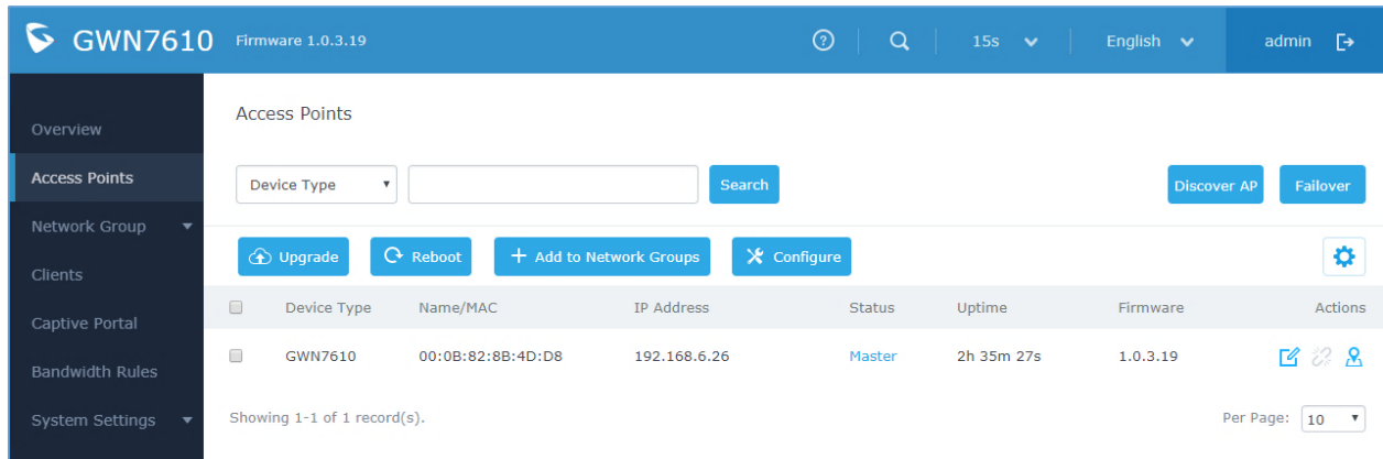
Figure 55: Access Points
