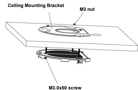
Figure 7: Ceiling Mount – Step 3
